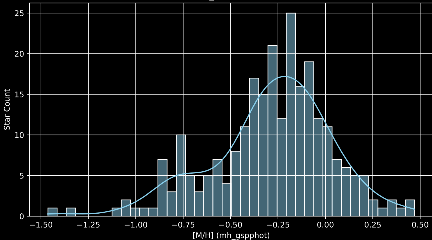
APOGEE DR17 Field: [K19_076+07_bt [M/H] (mh_gspphot) (n= 250)
