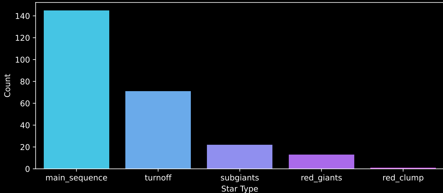
APOGEE DR17 Field: [K19_076+07_btx] Count plot of Star Type
