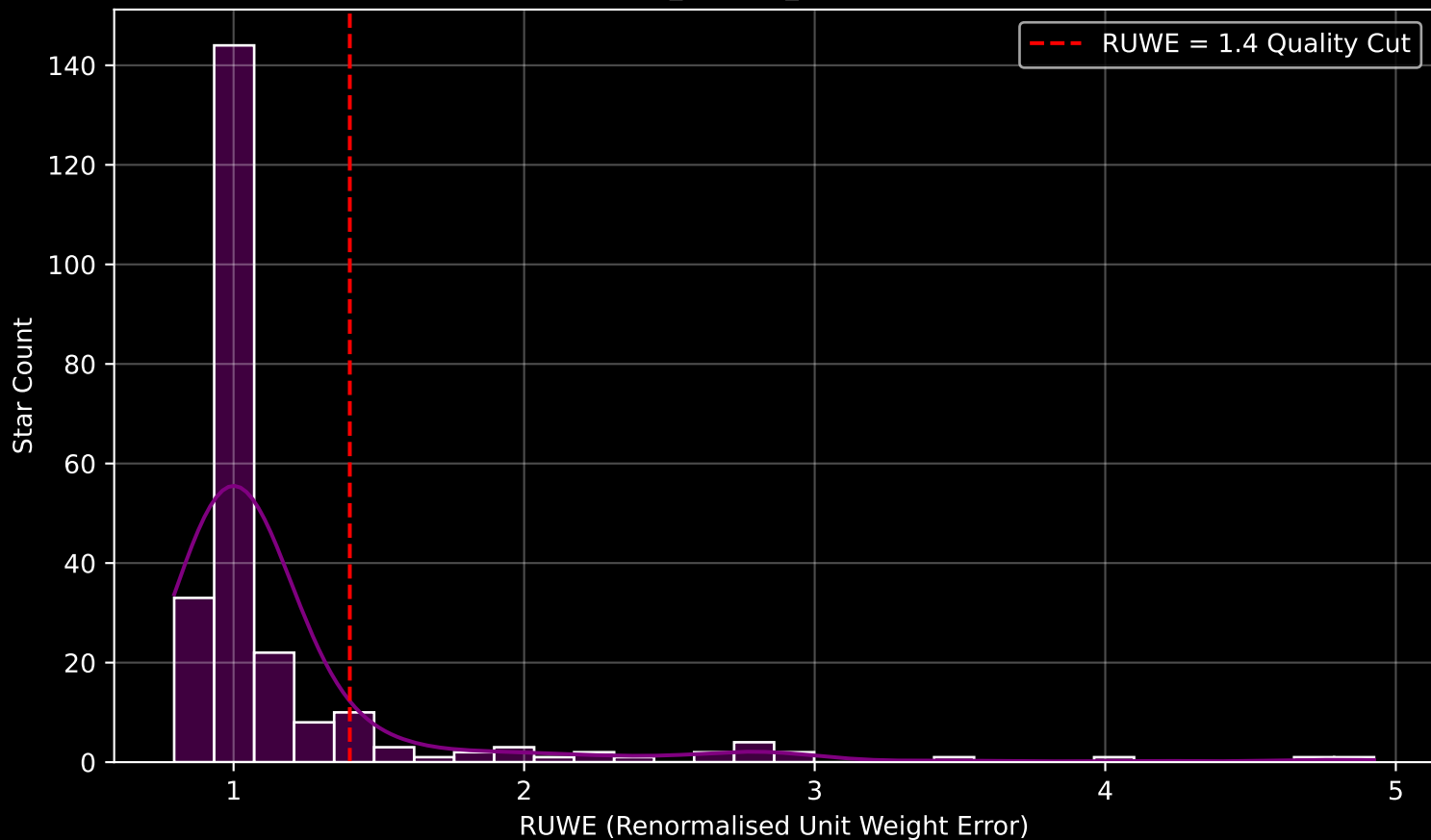
GAPOGEE DR17 Field [K19_076+07_btx] RUWE Distribution (n= 242)
