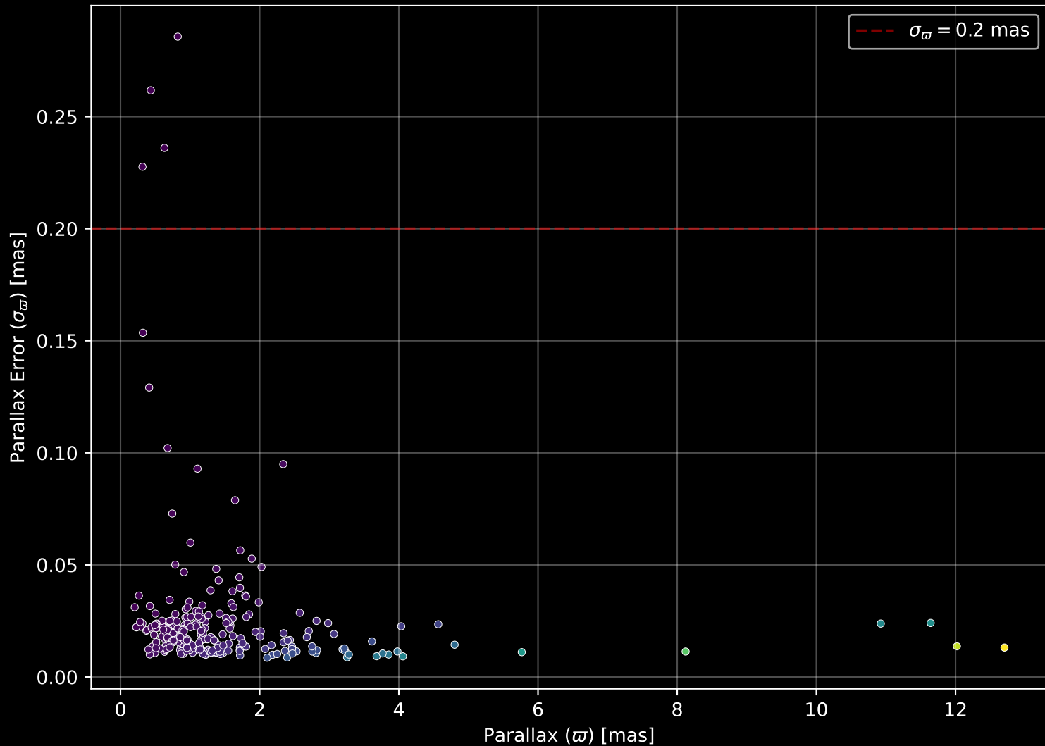
APOGEE DR17 Field: [K19_076+07_btx] Parallax Quality (n= 252)
