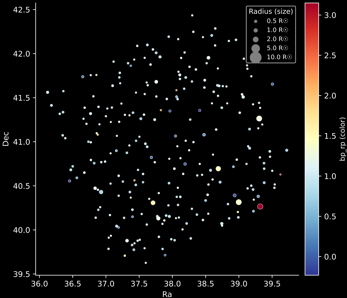
APOGEE DR17 Field: [K19_076+07_btx] Stars: 252
