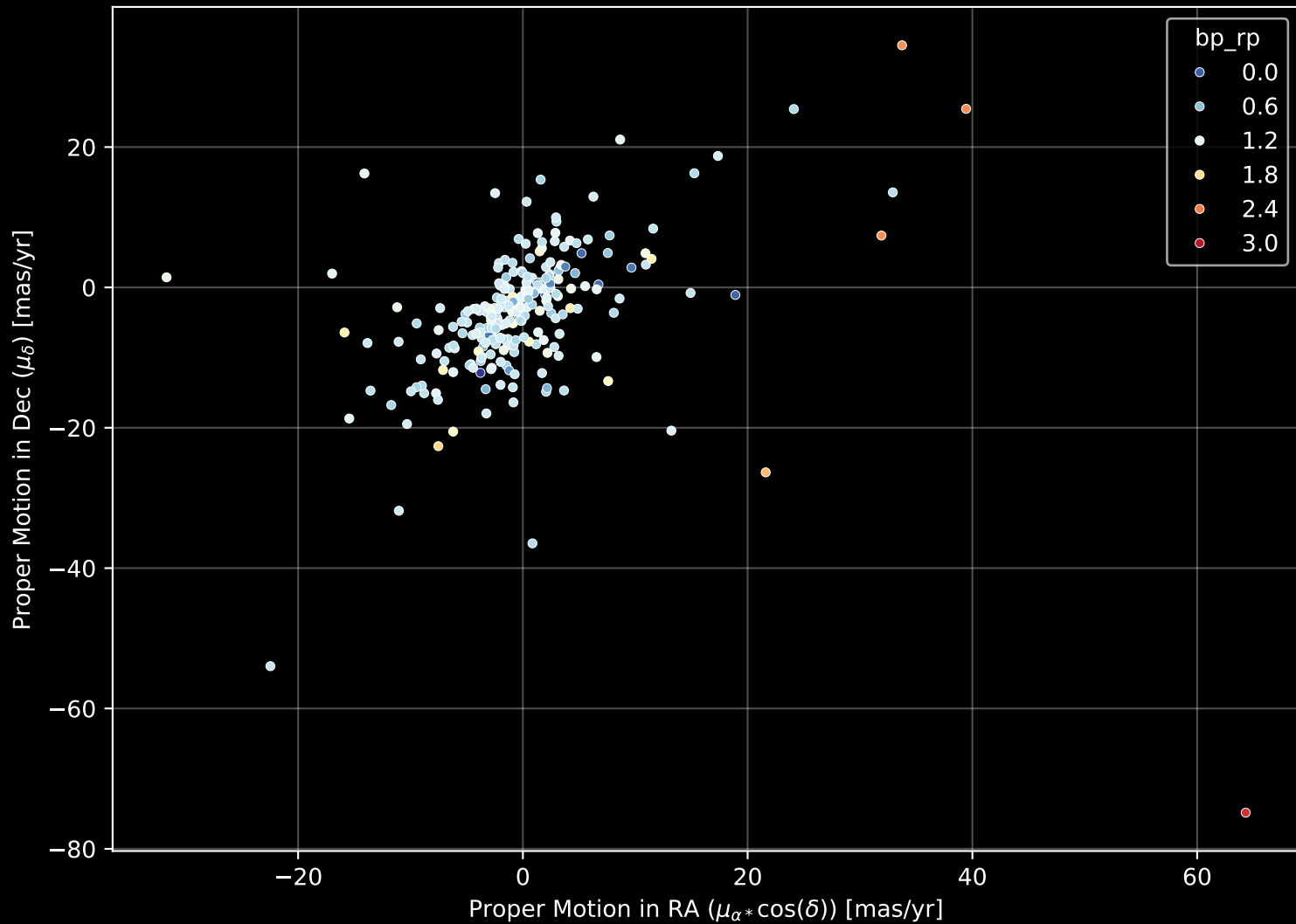
APOGEE DR17 Field: [K19_076+07_btx] Proper Motion Diagram (n= 252)
